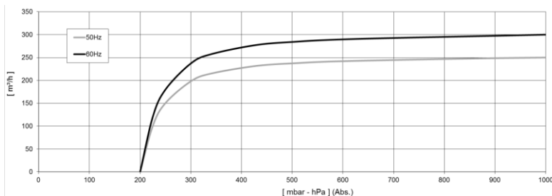
NOTE: Graph shows inlet pressure at a temperature of 68°F (tolerance ±10%)
