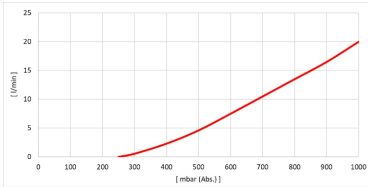
NOTE: Graph shows inlet pressure at a temperature of 68°F (tolerance ±10%)
