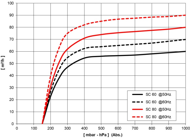
NOTE: Graph shows inlet pressure at a temperature of 68°F (tolerance ±10%)
